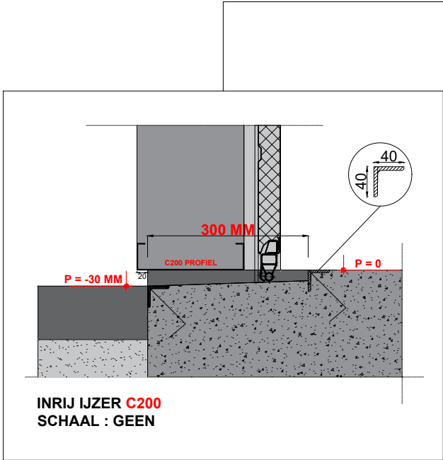
DETAIL WATERKERING
